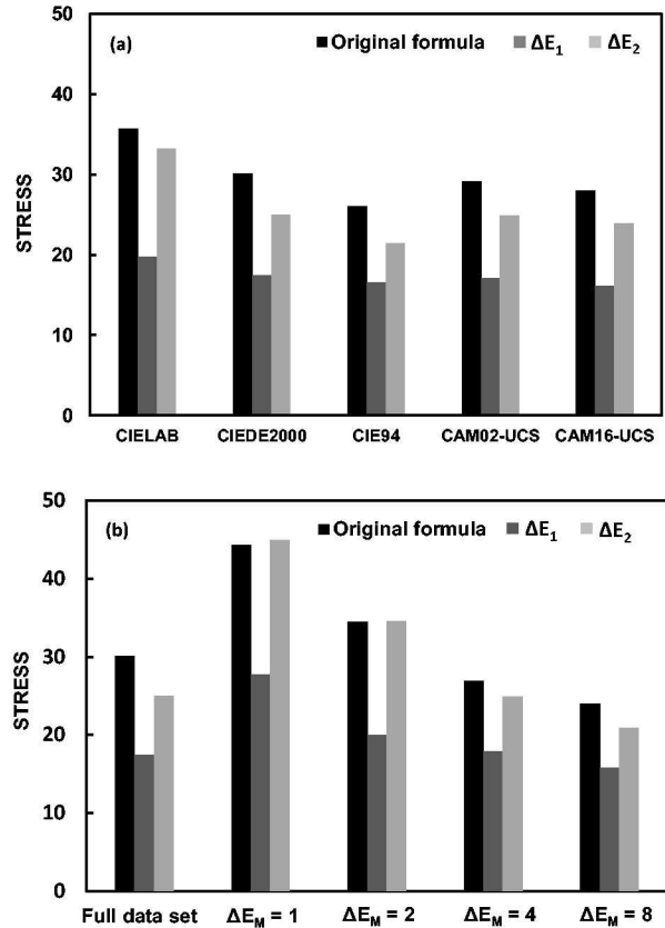
Figure 6. Performance of original, magnitude-corrected and power-corrected (a) colour difference formulae and (b) CIEDE2000 in terms of STRESS
