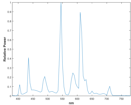
Figure 6 Spectral power distribution of test illuminant number 37 (F32T8/TL835 (1)) from the IES dataset for which R_f and MMCRI disagree and for which R_f is relatively high. The spectrum has numerous narrowband peaks with regions of very low power between them. R_f=80.6 and MMCRI = 53.0.
