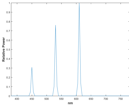
Figure 5 Spectral power distribution of test illuminant number 317 (Tri-band Gaussian) from the IES dataset for which R_f and MMCRI disagree. The spectrum contains three distinct spiky, very narrowband peaks with effectively zero power between the peaks. R_f=63.7 and MMCRI = 9.0
