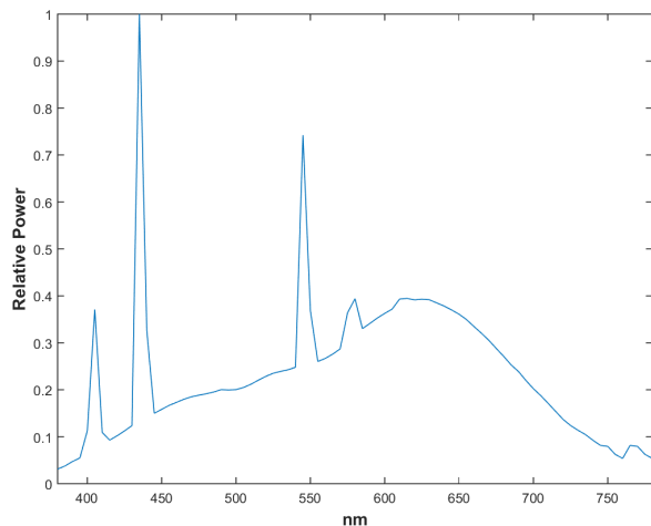
Figure 8 Spectral power distribution of test illuminant number 28 (F40T12/N (1)) from the IES dataset for which R_f and MMCRI agree. Although the spectrum has clear spikes, the tallest one is in a region of relatively low cone sensitivity and there are no near-zero values anywhere. R_f=85.8 and MMCRI=87.0 .
