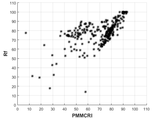
Figure 3. Comparison of the IES R_f color rendering index to PMMCRI.
