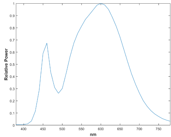
Figure 7 Spectral power distribution of test illuminant number 221 (LED Phosphor Blue Pump (53)) from the IES dataset for which R_f and MMCRI agree. The spectrum is smooth in comparison to those shown in Figures 5 and 6. It also contains no low values anywhere except at the very end of the visible spectrum. R_f=82.6 and MMCRI 85.1.
