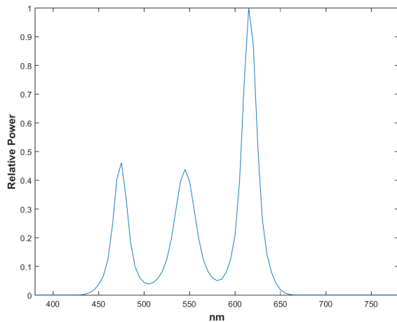
Figure 2. Spectral power distribution of test illuminant number #134 (RGB (474/545/616) Duv=-0.006) from the IES dataset having R_f = 74.2 and MMCRI = 40.8. The spectrum has three distinct peaks and low valleys.
