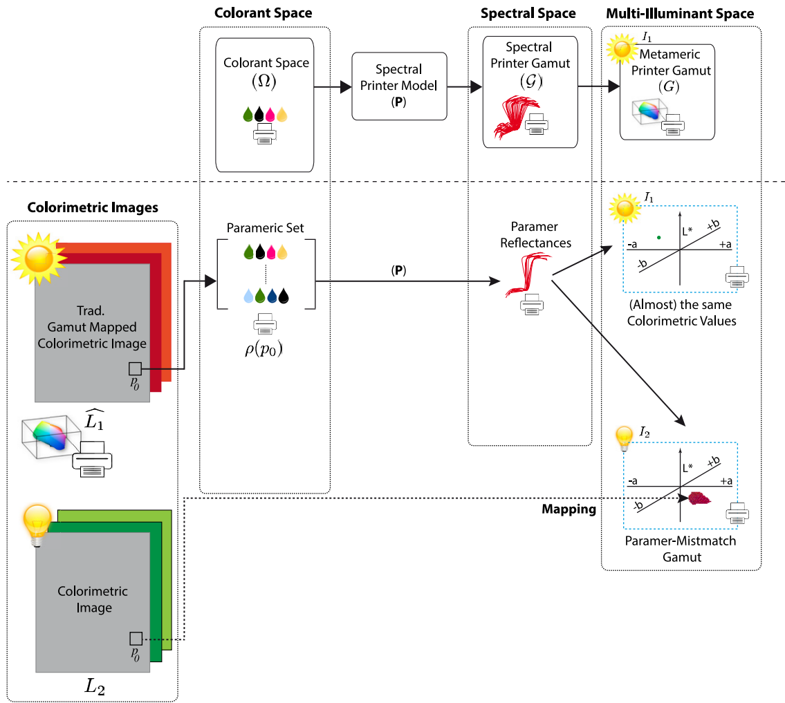
Figure 1. Schematic representation of the PMSGM framework—the fundamental of the proposed method in this article—in a multi-illuminant structure considering two illuminants.
