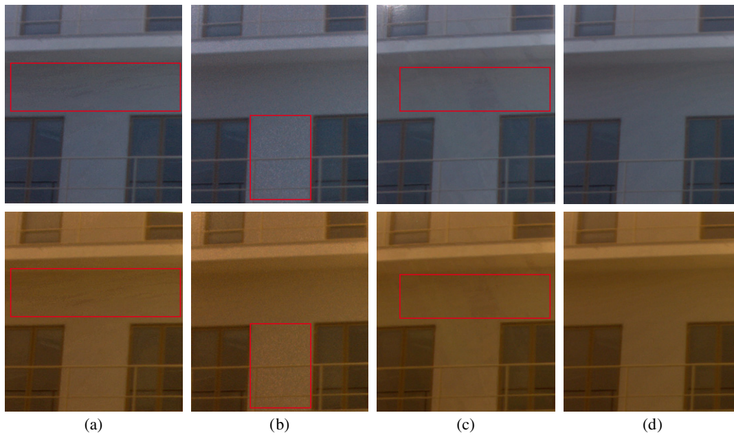
Figure 9. Cut-outs of captured images from spectral prints—based on the separations shown in Fig. 7—under the illuminants CIED65 (first row) and CIEA (second row). Different artifacts are visible in (a) (banding), (b) (graininess) and (c) (smearing), especially in the areas surrounded with red rectangles, while (d) shows the enhanced reproduction using the novel approach. It should be noted that the capture process can introduce color errors. The results are more reliable in the zoomed-in electronic version of the article.
