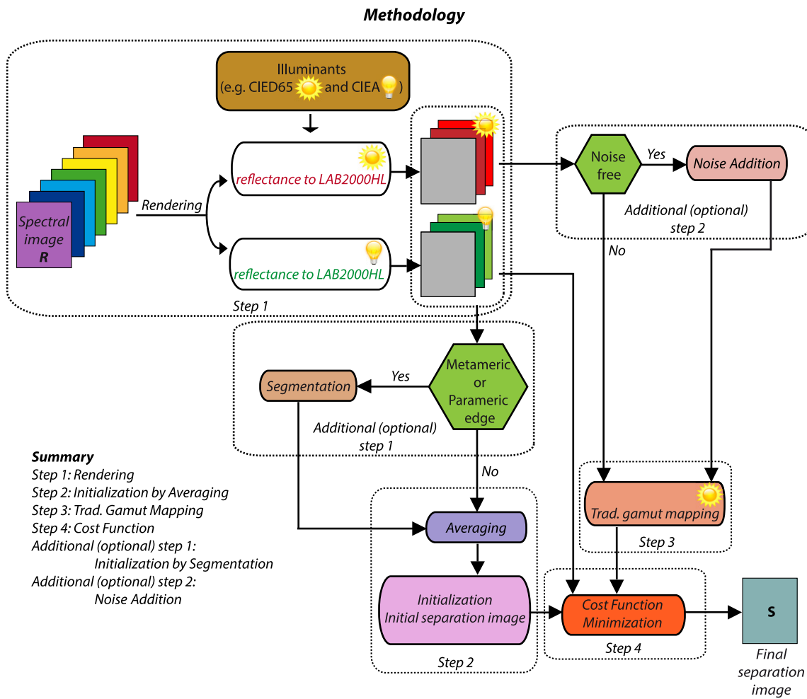
Figure 6. A block diagram representing the proposed methodology in an overall view.
