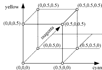
Figure 5. The subcube represents one of the 8 subcubes produced by the combinations of 0%, 50% and 100% surface coverages of the three inks. At the vertices (c,m,y) of the subcube, primary reflectances R_{c,m,y}(\lambda) have been measured.
