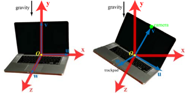
Figure 2: The xyz axes define a world coordinate system that is fixed with respect to gravity. The uvw axes define an object space coordinate system that is fixed with respect to landmarks on the laptop (the directions along the screen-base hinge, from the origin to the webcam, and origin to trackpad). Left, the two coordinate systems are aligned in the laptop's initial state. Right, the laptop has been rotated relative to the world coordinate system.
