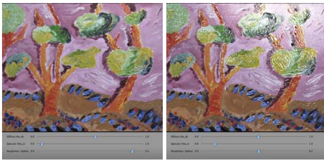
Figure 5: Dynamic control of material properties: The two renderings of the painting illustrate the tangiBook's ability to dynamically change the material properties of a displayed surface. The surface on the left has a relatively low specular reflectance ( \rho_s ) and a high roughness ( \alpha ) giving a matte appearance. Using the sliders, these two parameters have been altered in the surface on the right to produce glossy reflections.
