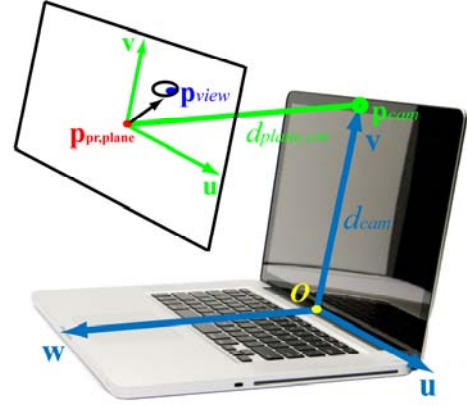
Figure 3: Diagram of the geometry for viewpoint tracking. The camera position ( \mathbf{p}_{cam} ) is located a known distance ( d_{cam} ) from the origin along the \mathbf{v} axis of the laptop coordinate system. The principal ray emanating from the camera points in the same direction as the \mathbf{w} axis. The point \mathbf{p}_{pr,plane} , where the principal ray intersects the perpendicular plane containing the eye-point, is found by moving along the principal ray a distance, d_{plane,cm} determined from the pinhole camera equation. The viewpoint ( \mathbf{p}_{view} ) is found by moving away from the intersection point in the \mathbf{u} and \mathbf{v} directions, based on the offset of the eye-point in the captured image relative to the image center.
