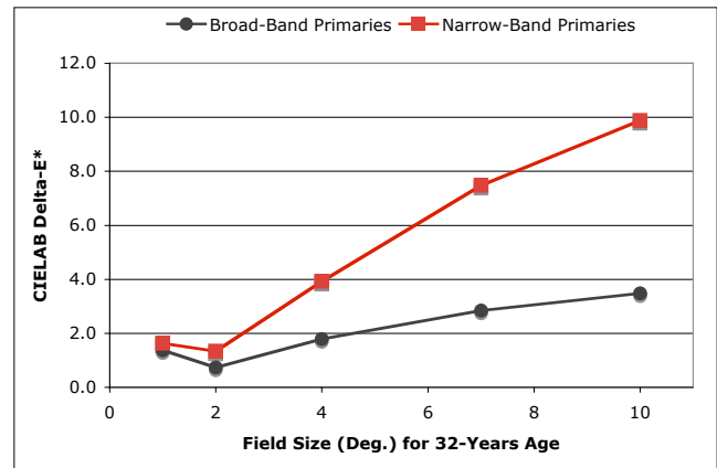
Figure 4. Mean CIELAB \Delta E^* (CIE 2^\circ ) between 24 ColorChecker patches under D65 and the simulated displays for CIE 2006 observers at age 32 with various field sizes.
