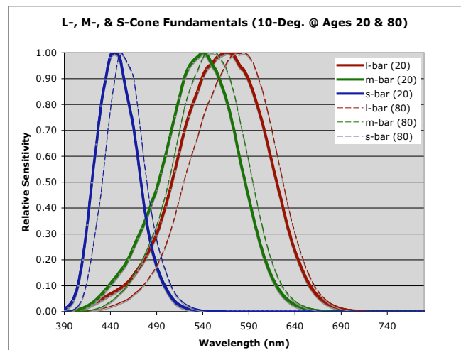
Figure 1. CIE 2006 cone fundamentals (color matching functions) for 2° and 10° field sizes at age 32 (upper panel) and ages 20 and 80 for a 10° field size (lower panel).
