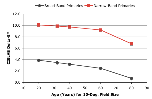
Figure 5. Mean CIELAB \Delta E^* (CIE 2^\circ ) between 24 ColorChecker patches under D65 and the simulated displays for CIE 2006 observers at various ages with 10^\circ field size.
