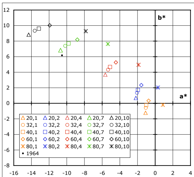
Figure 6. CIELAB a^*b^* values (CIE 2°) for the ColorChecker white patch when matched by various CIE 2006 color matching functions. Upper panel is for a broad-band-primary display while the lower panel is for a narrow-band-primary display. Note: The CIE 1931 2° observer would place both matches at a^*=b^*=0.0 .
