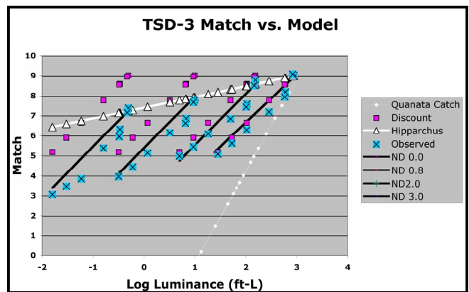
Figure 8 plots the black-surround physical description vs. observer data. The slope 3.8 predictions are the solid black lines. The Xs plot the observer data in four illumination levels. The fit is quite good. The triangles plot the low-slope Hipparchus line.
