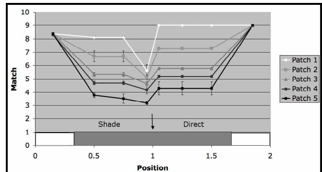
Figure 14 plots the matches along the rectangular patch for 5 target patches. The horizontal axis is the distance along the paper from white surround in shade to fold at the center and on to the white surround on the direct illumination side.
