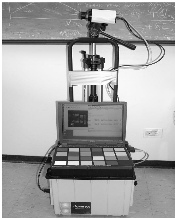
Figure 1. Portable high dynamic range imaging system
