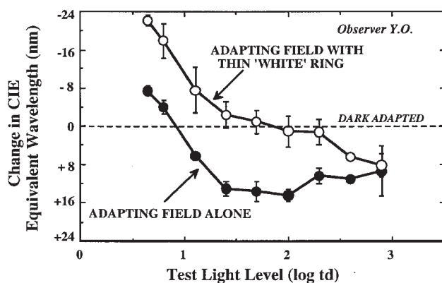
Figure 3. The change, relative to dark adaptation, in the spectral composition of a 1° test perceived as a 'perfect' (neither-reddish-nor-greenish) yellow (vertical axis), with the test on a 5°32 td 660 nm adapting field (filled symbols) or on the same 660 nm adapting field with an added thin achromatic ring of diameter 4°. Measurements were taken over a range of test-field levels (horizontal axis). Error bars indicate ± 1 standard error of the mean.
