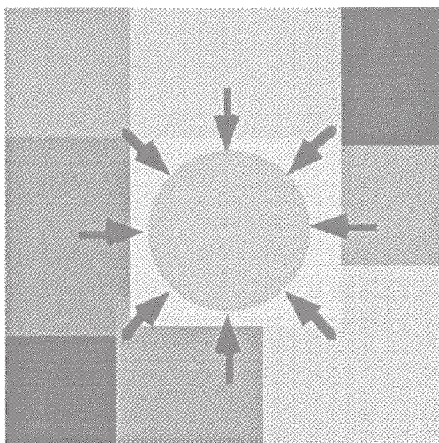
Figure 1. The appearance of the circle depends on contrast at its boundary (arrowheads) and on context. Context is defined as light outside of the circle that is beyond the boundary.
