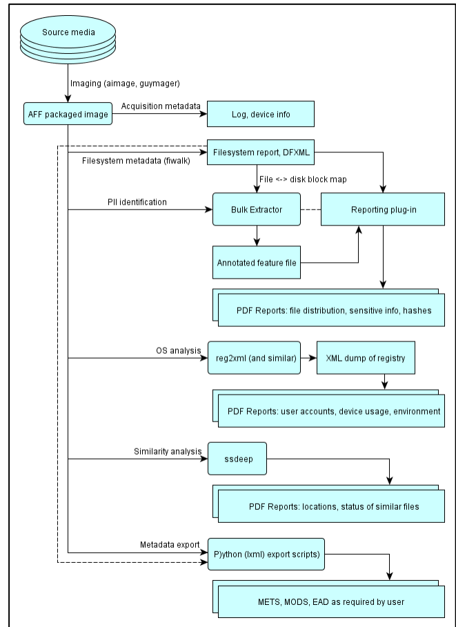
Figure 2: BitCurator architecture.
