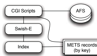
Figure 4. Metadata handling
