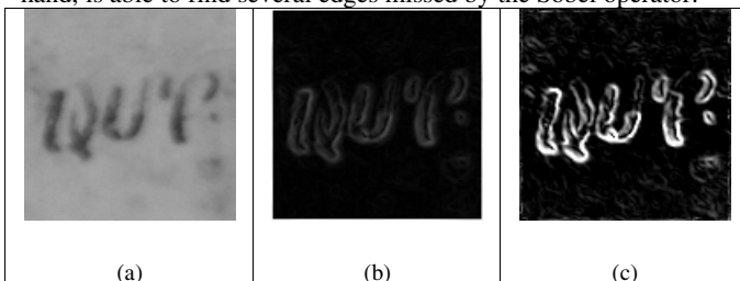
FIGURE 1: (a)Original image, (b)Output from Sobel Operator, (c)Output from proposed algorithm
