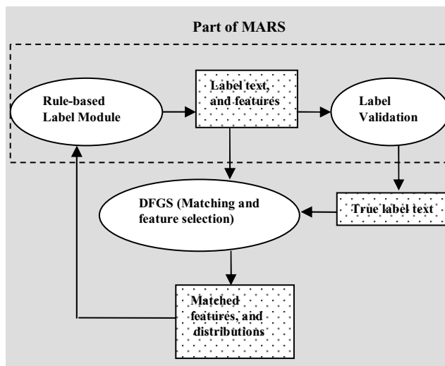
Figure 5. Dynamic Feature Generation System (DFGS) in MARS.
